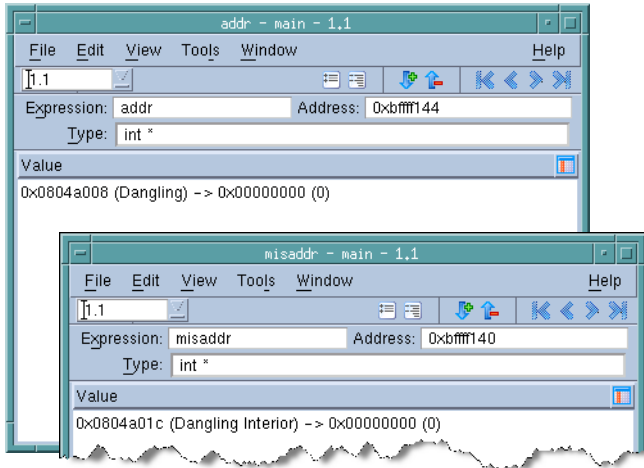
Figure 24 – Dangling Pointers
