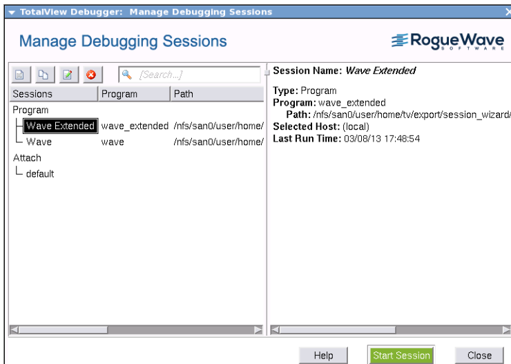
Figure 3 – Managing Sessions
