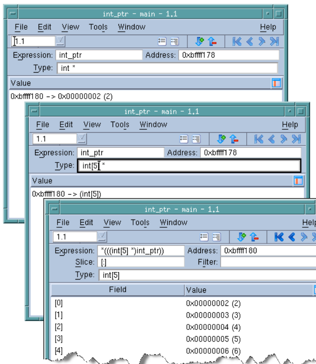
Figure 18 – Casting a Pointer to an Array
