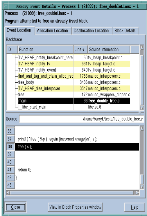
Figure 20 – Memory Block Event Window
