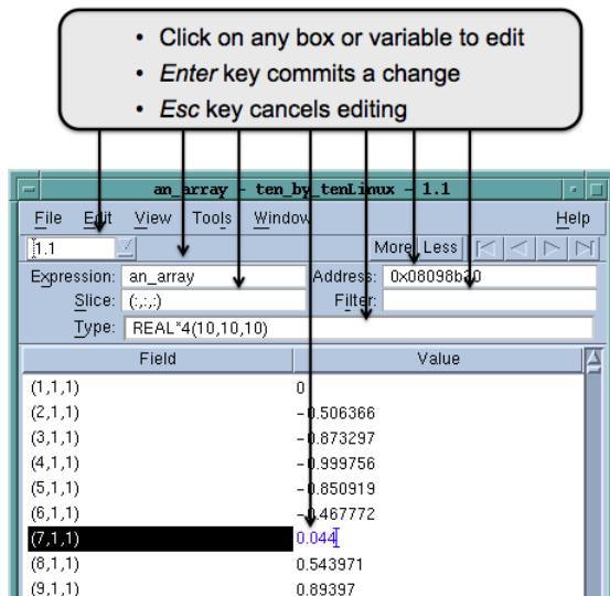
Figure 7 – Editing in the Variable Window
