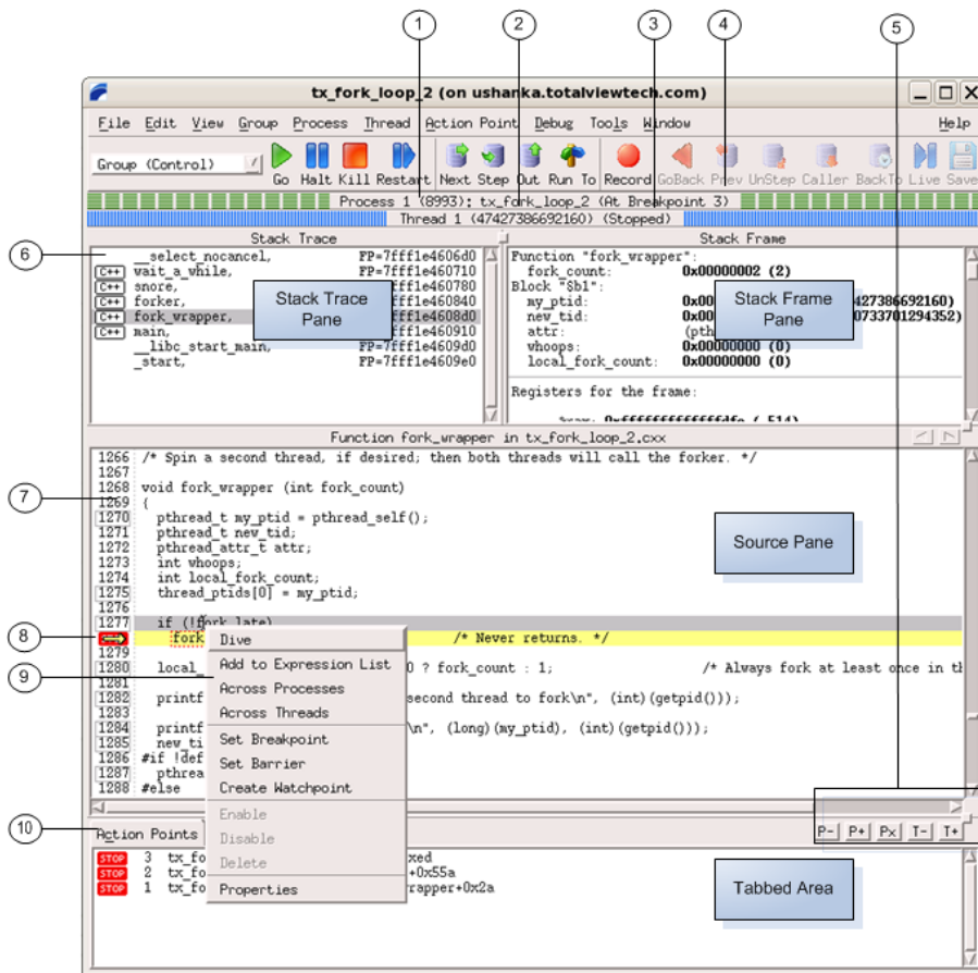
Figure 5 – A Process Window
