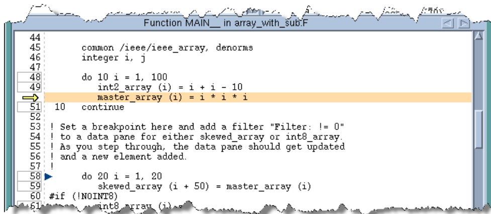
Figure 3 – Source Pane While ReplayEngine is in Replay Mode
